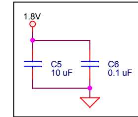
Place on DGND near PVDD
