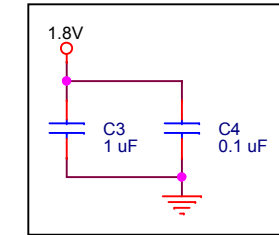
Place on DGND near PLL
