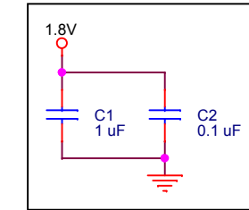
Place on DGND near DVDD_IO
